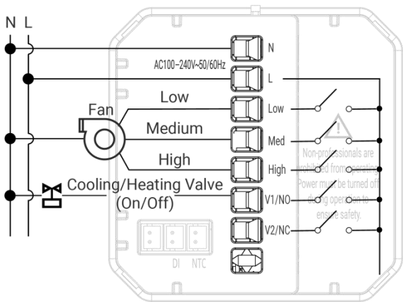
2-pipe, 2-wire ON/OFF valve, 3 speed fan
