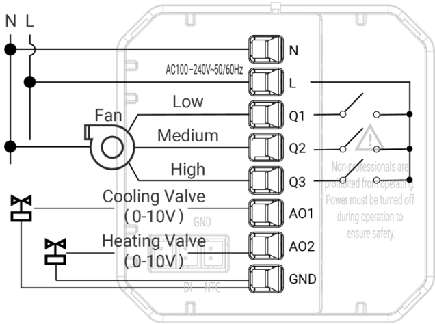
4-pipe, 0-10V valve, 3 speed fan
