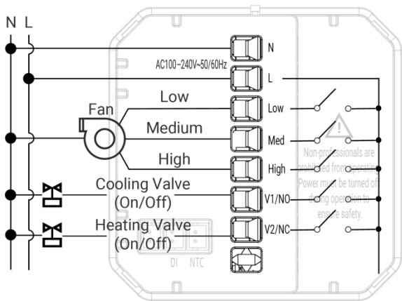
4-pipe, 2-wire ON/OFF valve, 3 speed fan
