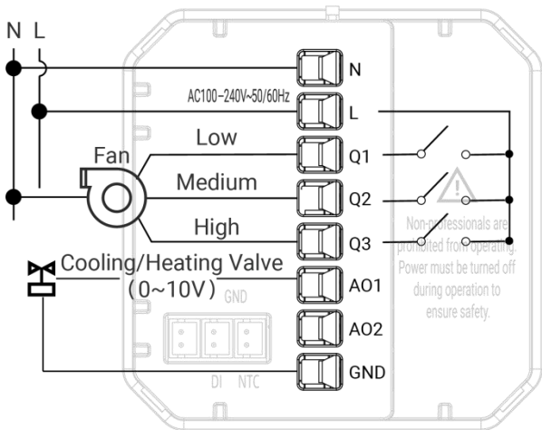
2-pipe, 0-10V valve, 3 speed fan
