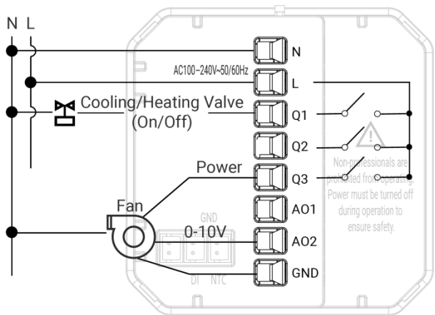
2-pipe, 2-wire ON/OFF valve, ECM fan
