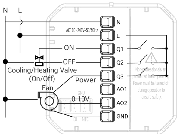
2-pipe, 3-wire ON/OFF valve, ECM fan
