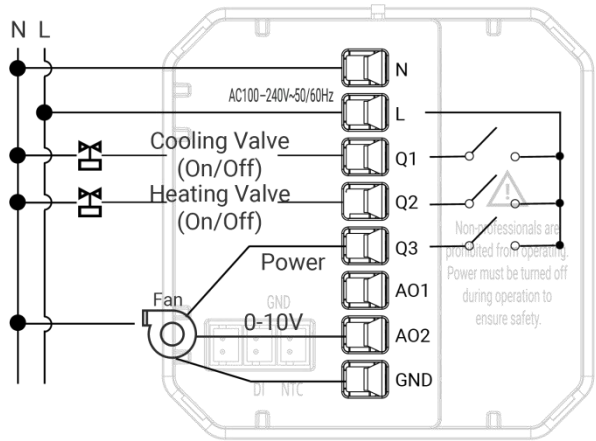
4-pipe, 2-wire ON/OFF valve, ECM fan
