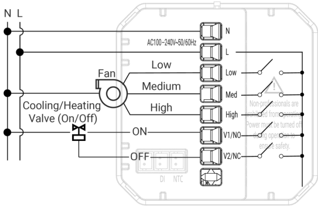
2-pipe, 3-wire ON/OFF valve, 3 speed fan
