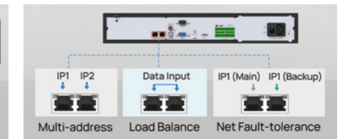
Dual Lan Giga Network Ports
