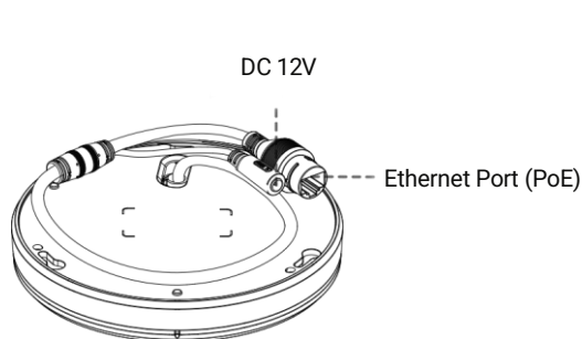
8MP Fisheye Camera
