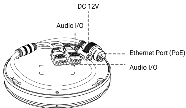
12MP Fisheye Camera
