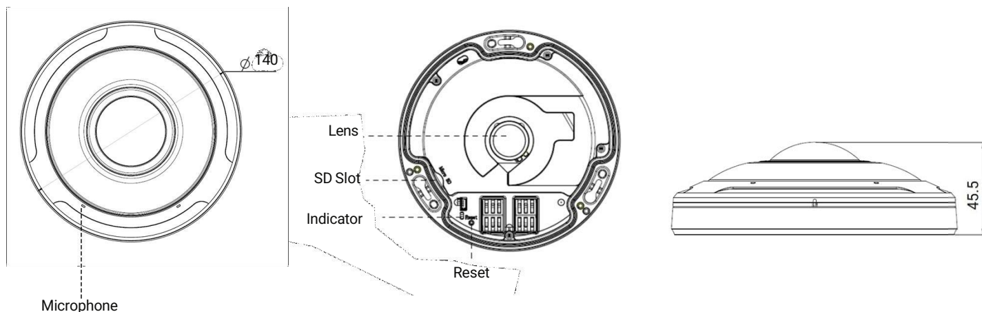
8MP Fisheye Camera (Multi-interface Version)
