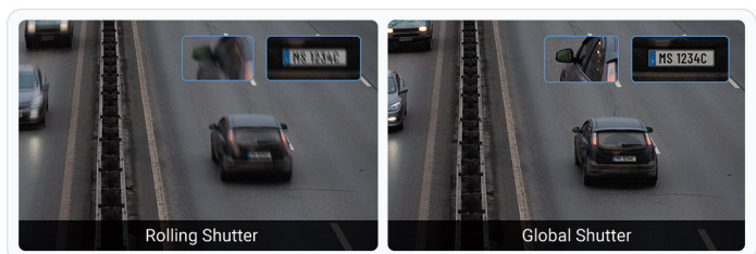
Global Shutter
