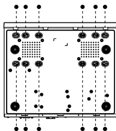
(Screw Position of 3.5" HDD)
