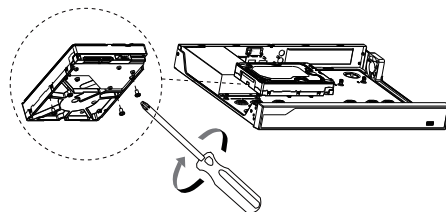
(3.5" HDD Installation)
